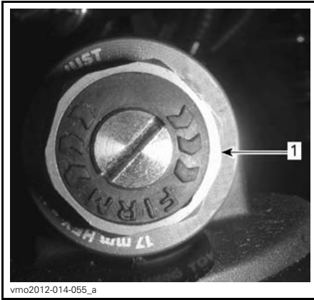
TYPICAL 1. High speed compression adjuster (17 mm wrench required)
