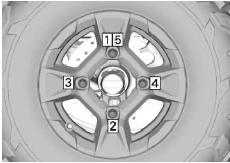
TIGHTENING SEQUENCE
