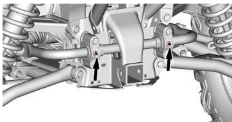
TYPICAL — REAR STABILIZER BAR
