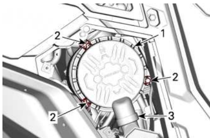
TYPICAL - RH SIDE OF VEHICLE, UNDER CARGO BOX
