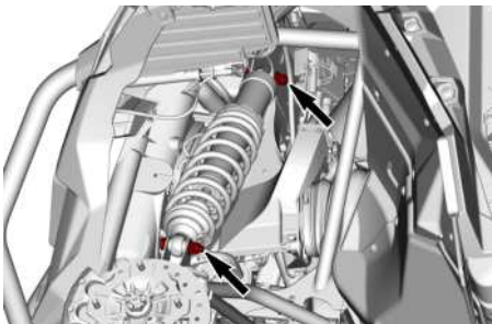
TYPICAL — FRONT SHOCK ABSORBER FASTENERS
