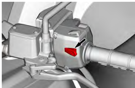
SET (ON)/DECEL-PAINIKE
