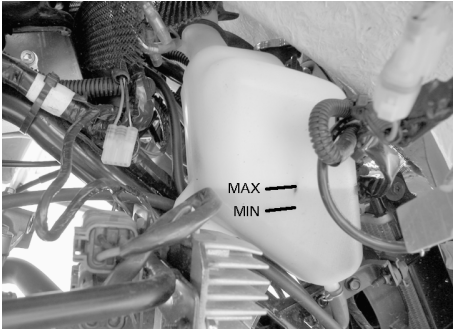
COOLANT LEVEL
