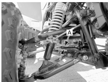
FRONT SUSPENSION
