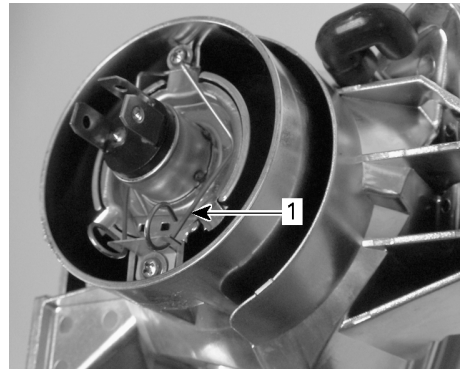
1. Retaining clip
