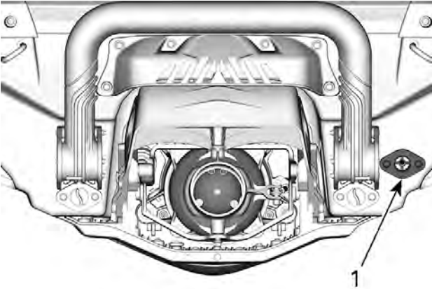
1. Flushing connector
