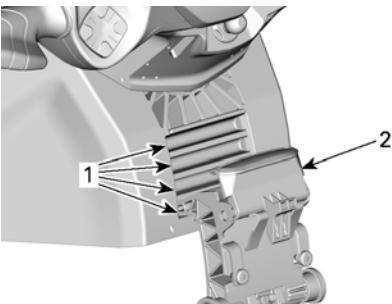
TYPICAL – STEERING COLUMN ADJUSTMENT LATCH SECURED 1. Steering support grooves 2. Release handle locked
