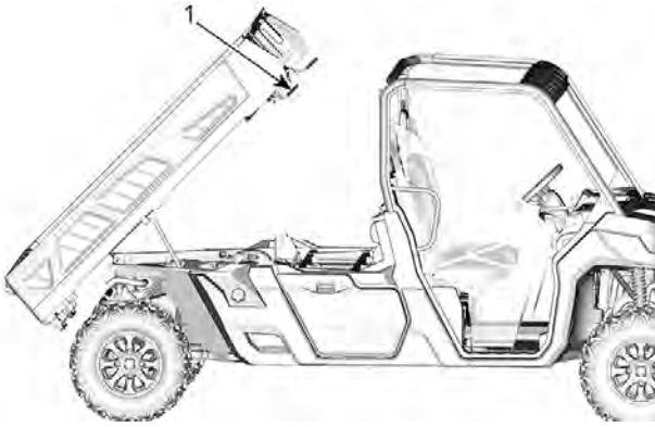
1. Release handles
