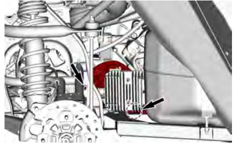
VOLTAGE/REGULATOR SUPPORT FASTENERS LOCATION
