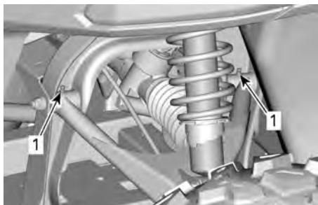
1. Smeefittingen ophangingsarm
