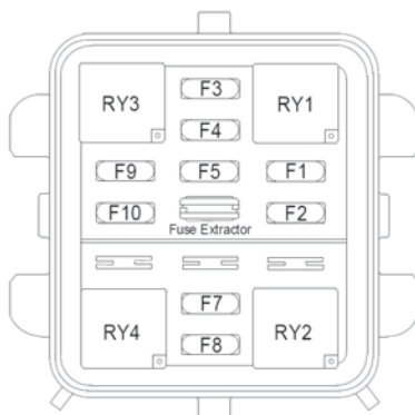
FB1-IDENTIFIERINGSDEKAL – 400 MM (16 TUM)
