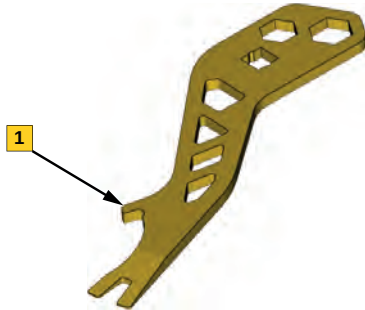
1. Suspension adjustment teeth.
