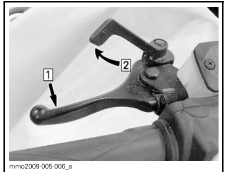
mmo2009-005-006_a TYPICAL — ENGAGE MECHANISM Step 1: Apply and hold regular brake Step 2: Lock brake lever using parking brake lever
